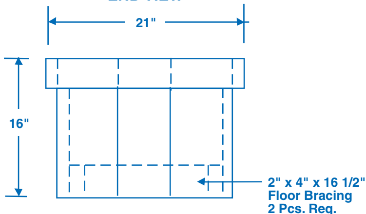
END VIEW
